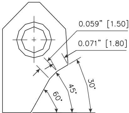
RCA043 Carbide Seat Insert 30-45-60 / 18 -15
