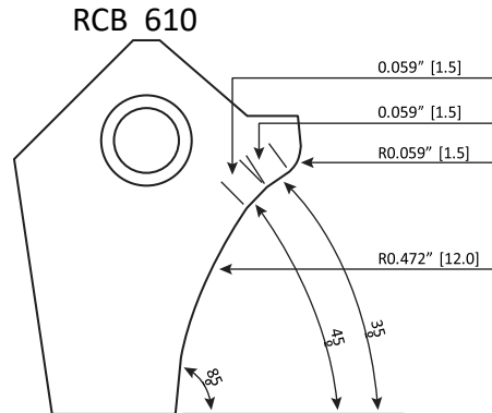
RCB610 Carbide Seat Insert R15-35-45-R122-85 / 18-15-15-30
