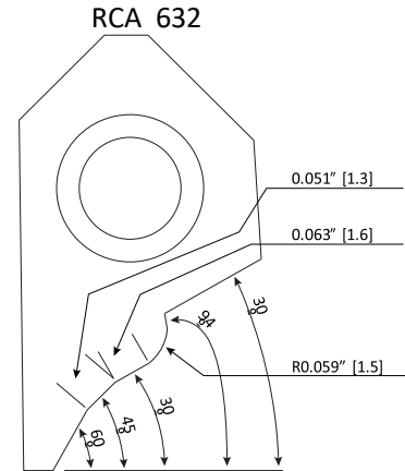
RCA632 Carbide Seat Insert 30-94-R15-30-45-60 / 16-13
