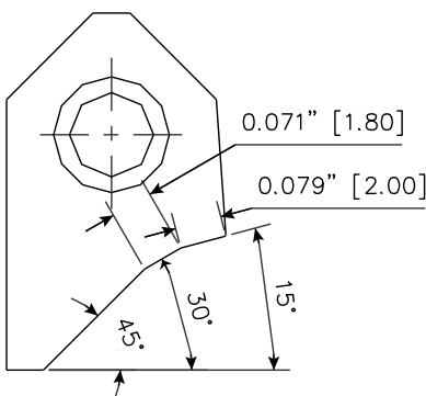
RCA312 Carbide Seat Insert 15-30-45 / 20 -18 RCA-312
