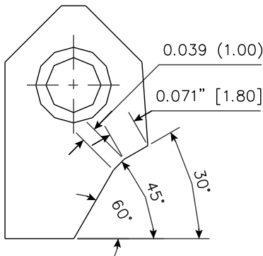
RCA056 Carbide Seat Insert 30-45-60 / 18 -10 RCA-056
