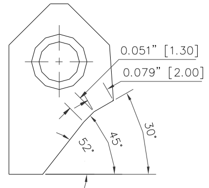
RCA006 Carbide Seat Insert 30-45-52 / 20 -13
