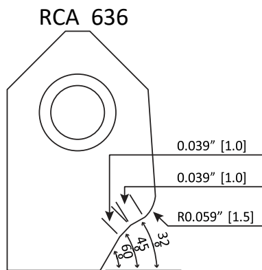
RCA636 Carbide Seat Insert R15-32-45-60 / 16-10-10 (Offset Bit)
