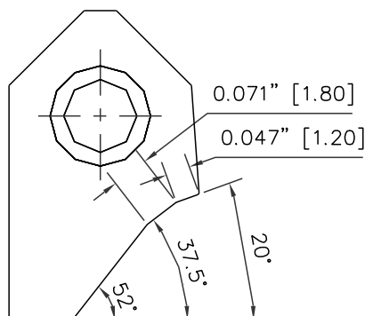
RCA406 Carbide Seat Insert 20-375 -52 / 12 -18
