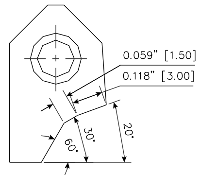
RCA325 Carbide Seat Insert 20-30-60 / 30 -15 RCA-325
