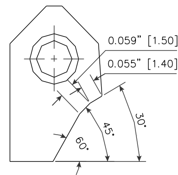
RCA044 Carbide Seat Insert 30-45-60 / 14 -15
