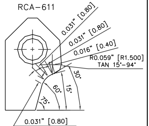
RCA611 Carbide Seat Insert R15-15-30-45-60-75 / 22-08
