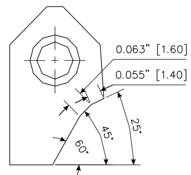
RCA045 Carbide Seat Insert 25-45-60 / 14 -16
