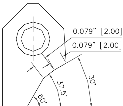
RCA403 Carbide Seat Insert 30-375 -60 / 20 -20
