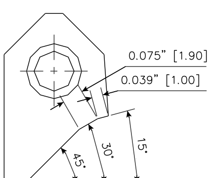
RCA313 Carbide Seat Insert 15-30-45 / 10 -19 RCA-313
