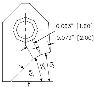
RCA309 Carbide Seat Insert 15-30-45 / 20 -16 RCA-309
