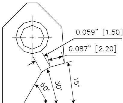
RCA324 Carbide Seat Insert 15-30-60 / 22 -15 RCA-324
