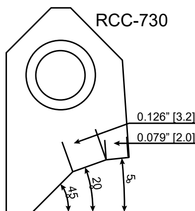
RCC730 C Blank Carbide Seat Insert 5-20-45 / 20-32
