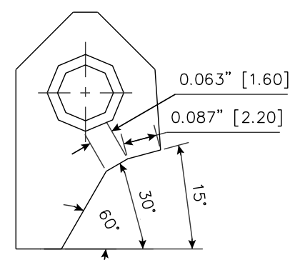
RCA311 Carbide Seat Insert 15-30-60 / 22 -16 RCA-311
