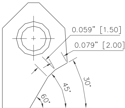
RCA010 Carbide Seat Insert 30-45-60 / 20 -15 RCA-010
