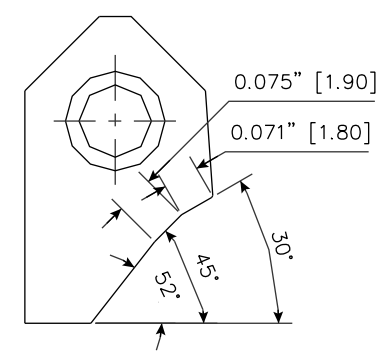
RCA027 Carbide Seat Insert 30-45-52 / 18 -19 RCA-027
