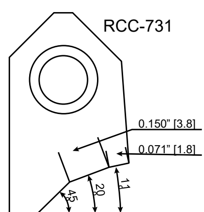
RCC731 C Blank Carbide Seat Insert 11-20-45 / 18-38
