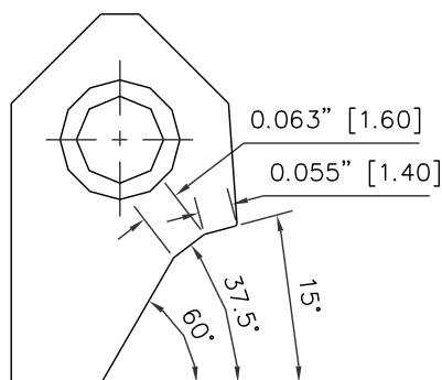
RCA405 Carbide Seat Insert 15-375 -60 / 14 -16
