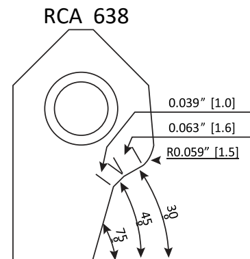
RCA638 Carbide Seat Insert R15-30-45-75 / 16-10
