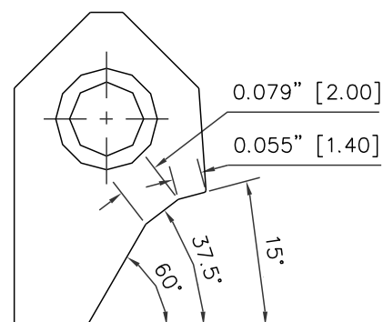
RCA407 Carbide Seat Insert 15-375 -60 / 14 -16
