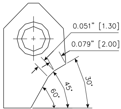
RCA042 Carbide Seat Insert 30-45-60 / 10 -14
