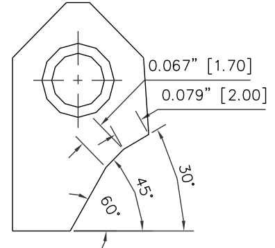
RCA048 Carbide Seat Insert 30-45-60 / 20 -17 RCA-048
