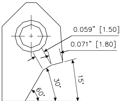
RCA323 Carbide Seat Insert 15-30-60 / 18 -15 RCA-323
