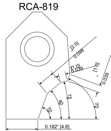
RCA819 Carbide Seat Insert 15- 40-70 with 70 degree radius top, - 10-25
