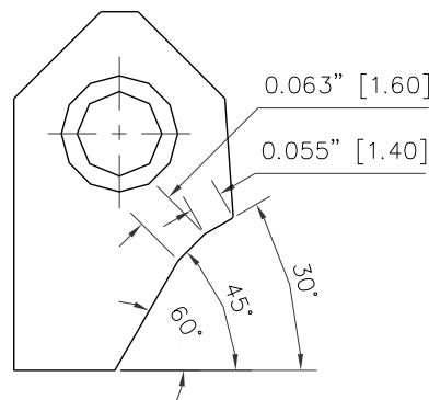
RCA014 Carbide Seat Insert 30-45-60 / 14 -16 RCA-014
