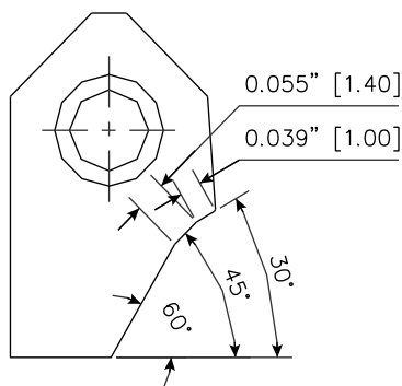
RCA040 Carbide Seat Insert 30-45-60 / 20 -13
