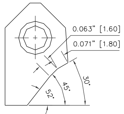
RCA018 Carbide Seat Insert 30-45-52 / 18 -16 RCA-018
