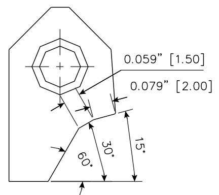
RCA305 Carbide Seat Insert 15-30-60 / 20 -15 RCA-305
