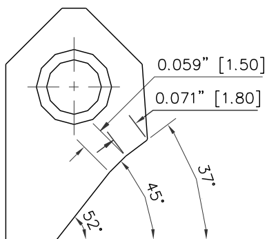
RCA007 Carbide Seat Insert 37-45-52 / 18 -15
