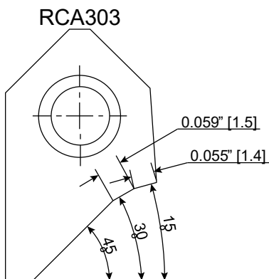
RCA303 Carbide Seat Insert 15-30-45 / 14 -15
