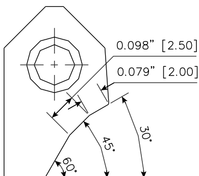
RCA034 Carbide Seat Insert 30-45-60 / 20 -25
