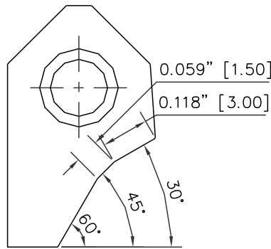
RCA011 Carbide Seat Insert 30-45-60 / 30 -15 RCA-011
