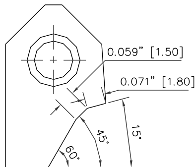
RCA008 Carbide Seat Insert 15-45-60 / 18 -15
