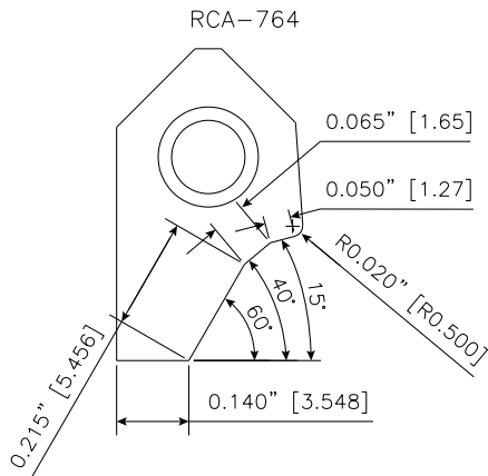
RCA764 Carbide Seat Insert 15- 40-60 top, seat width 127-165
