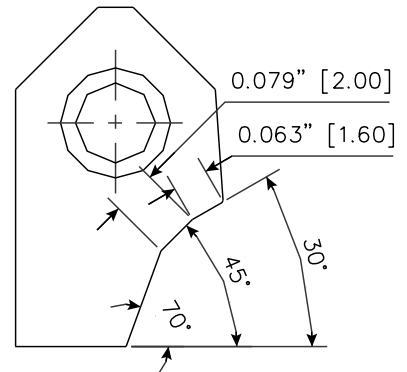
RCA030 Carbide Seat Insert 30-45-70 / 16 -20
