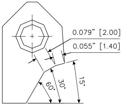
RCA326 Carbide Seat Insert 15-30-60 / 14 -20 RCA-326
