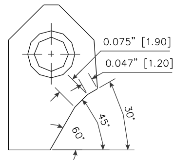
RCA025 Carbide Seat Insert 30-45-60 / 12 -19 (Caterpillar 3500E Intake seat Profile) RCA-025
