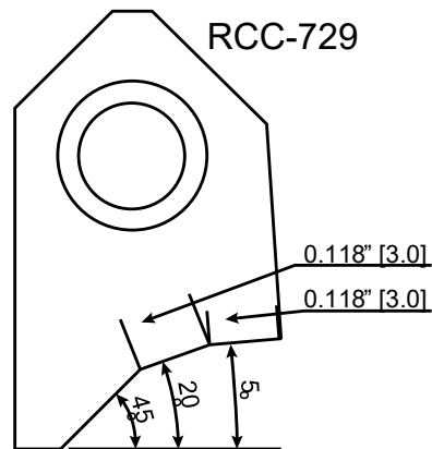
RCC729 C Blank Carbide Seat Insert 5-20-45 / 30-30
