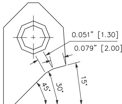
RCA301 Carbide Seat Insert 15-30-45 / 20 -13 RCA-301
