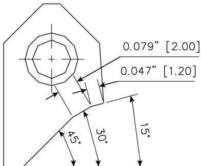
RCA315 Carbide Seat Insert 15-30-45 / 12 -20 (Caterpillar 3500E Exhaust seat Profile) RCA-315
