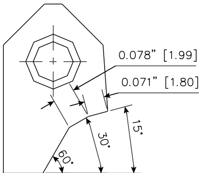
RCA327 Carbide Seat Insert 15-30-60 / 18 -20 RCA-327
