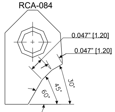
RCA084 Carbide Seat Insert 30-45-60 / 12-12
