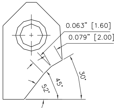
RCA020 Carbide Seat Insert 30-45-52 / 20 -16 RCA-020
