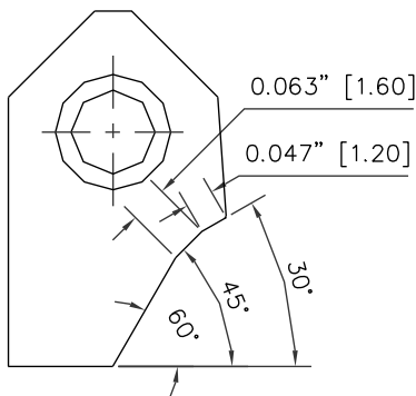
RCA013 Carbide Seat Insert 30-45-60 / 12 -16 RCA-013
