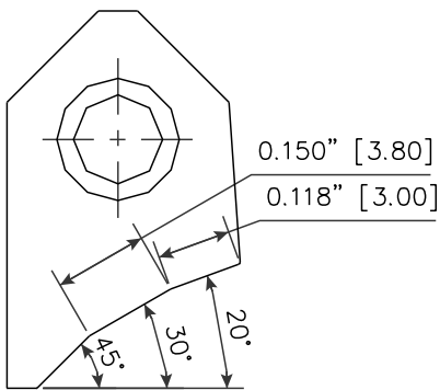
RCA318 Carbide Seat Insert 20-30-45 / 30 -38 RCA-318
