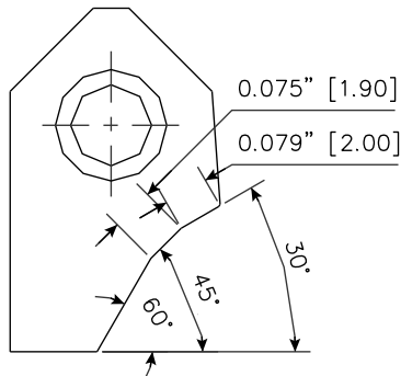
RCA029 Carbide Seat Insert 30-45-60 / 20 -19
