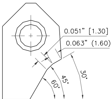
RCA004 Carbide Seat Insert 30-45-60 / 16 -13
