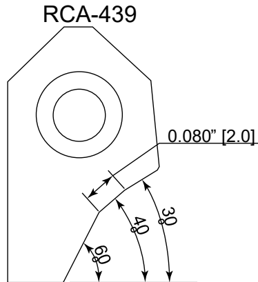
RCA439 Carbide Seat Insert 30-40-60 top, seat width 080
