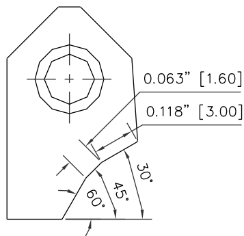
RCA022 Carbide Seat Insert 30-45-60 / 30 -16 RCA-022
