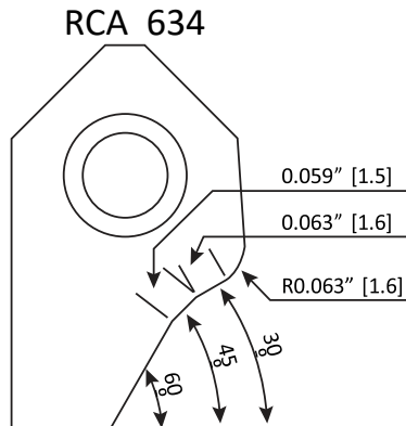
RCA634 Carbide Seat Insert R16-30-45-60 / 16-15
