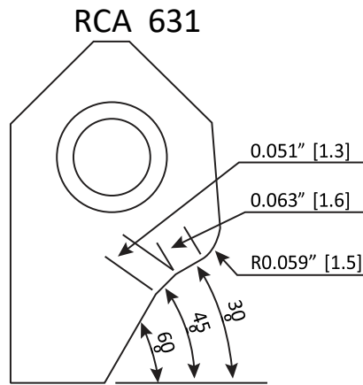
RCA631 Carbide Seat Insert R15-30-45-60 / 16-13
