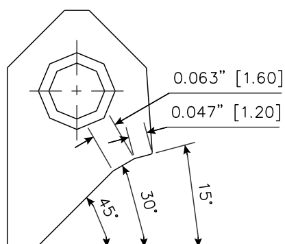
RCA306 Carbide Seat Insert 15-30-45 / 12 -16 RCA-306
