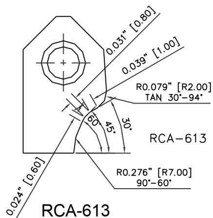
RCA613 Carbide Seat Insert R2- 30-45-60-R7 / 19-08
