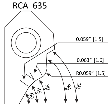
RCA635 Carbide Seat Insert 30-94-R15-30-45-60 / 16-15
