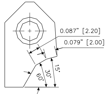
RCA317 Carbide Seat Insert 15-30-60 / 20 -22 RCA-317
