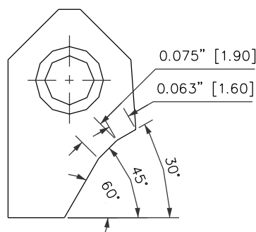
RCA026 Carbide Seat Insert 30-45-60 / 16 -19 RCA-026
