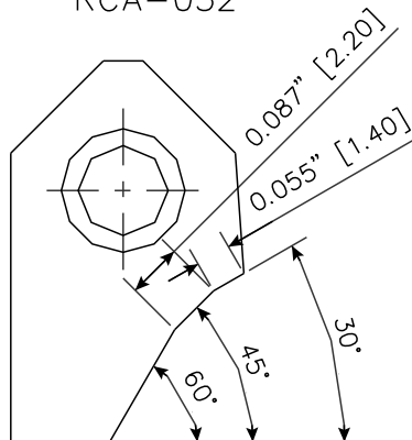
RCA032 Carbide Seat Insert 30-45-60 / 06 -22
