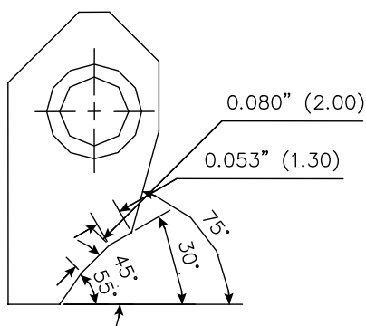
RCA062 Carbide Seat Insert 30-45-55 / 13-20
