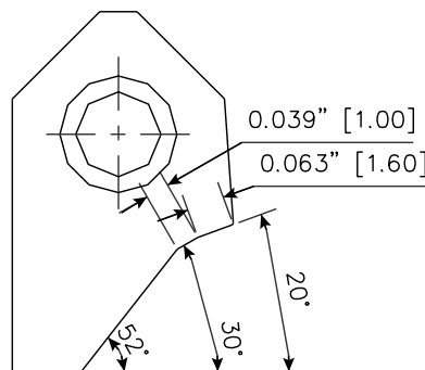
RCA321 Carbide Seat Insert 20-30-52 / 16 -10 RCA-321
