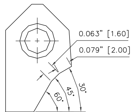
RCA021 Carbide Seat Insert 30-45-60 / 20 -16 RCA-021
