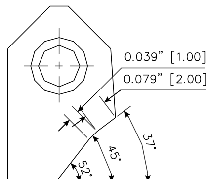
RCA057 Carbide Seat Insert 37-45-52 / 20 -10 RCA-057
