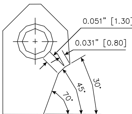
RCA070 Carbide Seat Insert 30-45-70 / 80-13 RCA-070
