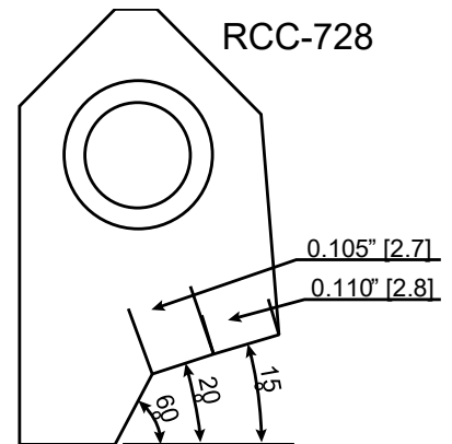
RCC728 C Blank Carbide Seat Insert 15-20-60 / 28-266
