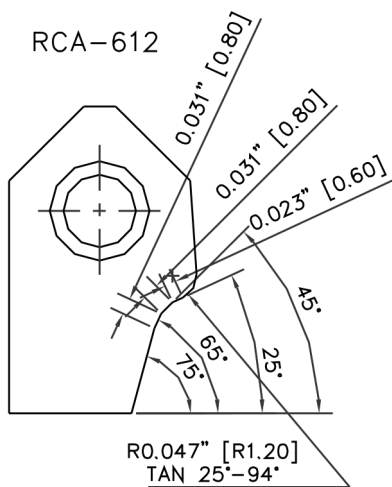
RCA612 Carbide Seat Insert R12-25-45-65-75 / 12-08
