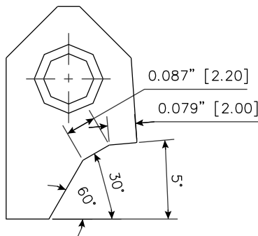
RCA333 Carbide Seat Insert 5-30-60 / 20 -22 (Cummins NH Series Cylinder Head) RCA-333
