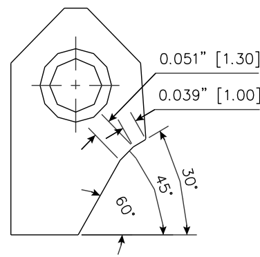
RCA041 Carbide Seat Insert 30-45-60 / 10 -13
