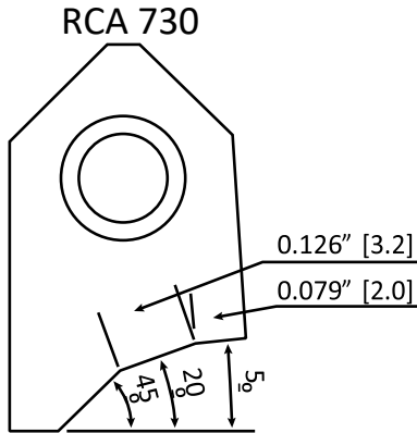
RCA730 Carbide Seat Insert 5-20-45 / 20mm - 32mm (126")
