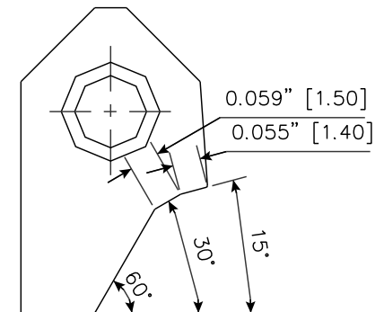
RCA334 Carbide Seat Insert 15-30-60 / 14-15 RCA-334
