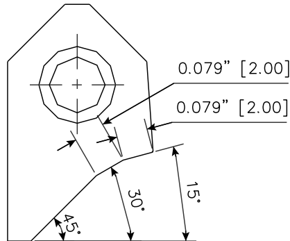
RCA316 Carbide Seat Insert 15-30-45 / 20 -20 RCA-316
