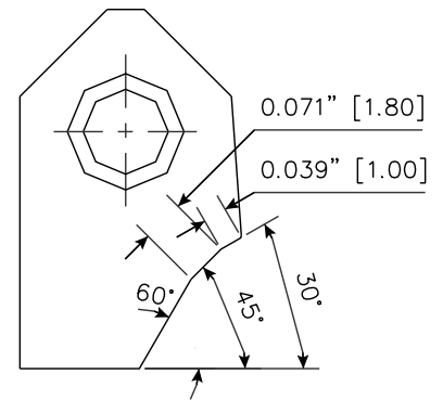
RCA075 Carbide Seat Insert 30-45-60 / 10-18 RCA-075
