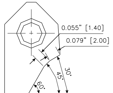
RCA081 Carbide Seat Insert 30-45-60 / 20-14 RCA-081
