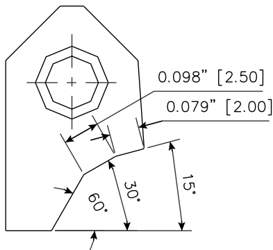
RCA329 Carbide Seat Insert 15-30-60 / 20 -25 RCA-329
