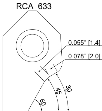
RCA633 Carbide Seat Insert 30-45-60 / 20-14
