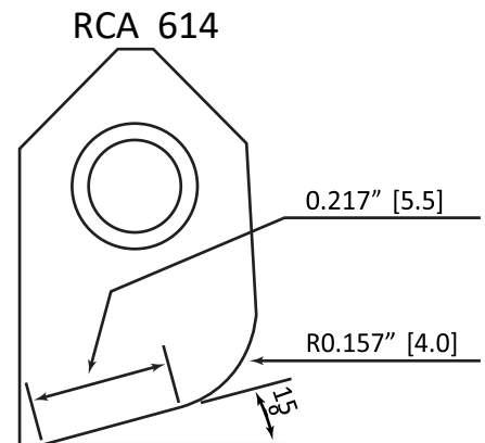
RCA614 Carbide Seat Insert R4 -15 / 552mm
