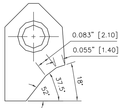
RCA404 Carbide Seat Insert 18-375 -52 / 06 -21
