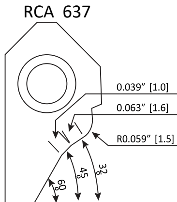
RCA637 Carbide Seat Insert R15-32-45-60 / 16-10-10
