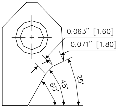
RCA046 Carbide Seat Insert 25-45-60 / 18 -16 RCA-046
