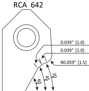
RCA642 Carbide Seat Insert R15-20-45-60 / 10-10
