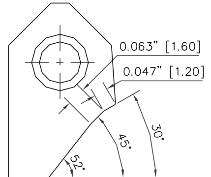
RCA012 Carbide Seat Insert 30-45-52 / 12 -16 RCA-012
