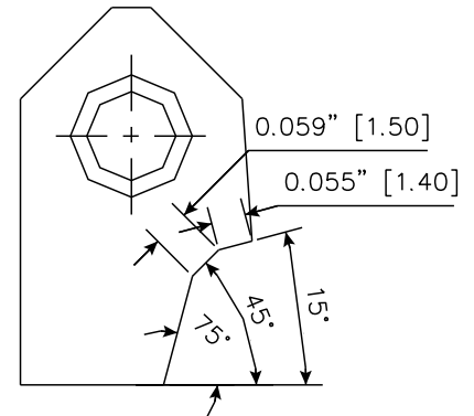
RCA078 Carbide Seat Insert 12-45-75 / 14-15 RCA-078
