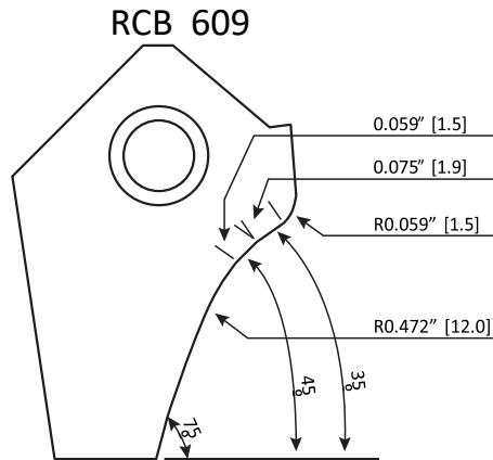
RCB609 Carbide Seat Insert R15-35-45-R12-75 / 19-15-25-30
