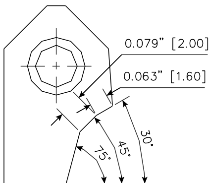
RCA031 Carbide Seat Insert 30-45-75 / 16 -20
