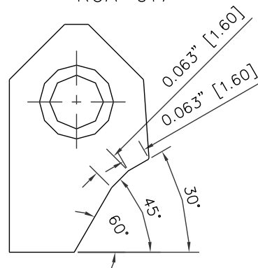
RCA017 Carbide Seat Insert 30-45-60 / 20 -22 RCA-017
