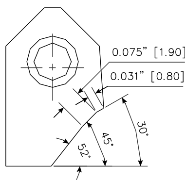
RCA050 Carbide Seat Insert 30-45-52 / 08 -19 RCA-050
