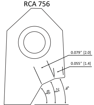
RCA756 Carbide Seat Insert For CAT C9 Engines
