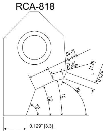
RCA818 Carbide Seat Insert 15- 25-70 with 70 degree radius top, - 15-30
