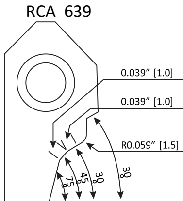
RCA639 Carbide Seat Insert 30R15-30-45-75 / 10-10
