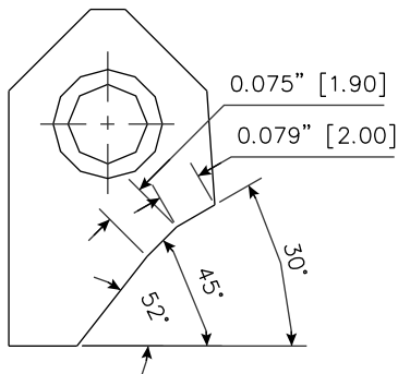
RCA028 Carbide Seat Insert 30-45-52 / 20 -19
