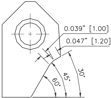
RCA001 Carbide Seat Insert 30-45-60 / 12 -10
