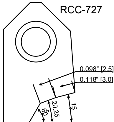
RCC727 C Blank Carbide Seat Insert 15-2025-60 / 30-25
