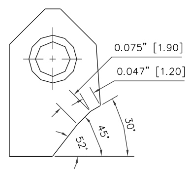
RCA024 Carbide Seat Insert 30-45-52 / 12 -19 RCA-024
