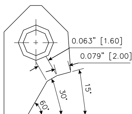
RCA310 Carbide Seat Insert 15-30-60 / 20 -16 RCA-310
