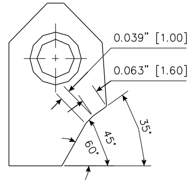
RCA039 Carbide Seat Insert 35-45-60 / 16 -10
