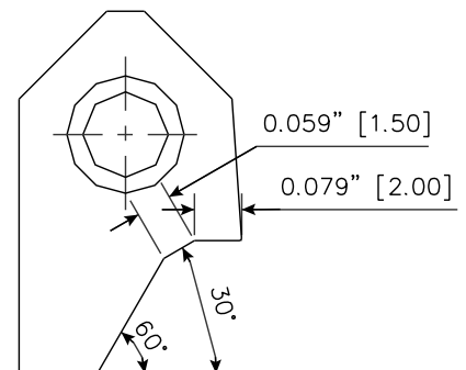
RCA322 Carbide Seat Insert 0-30-60 / 20 -15 RCA-322
