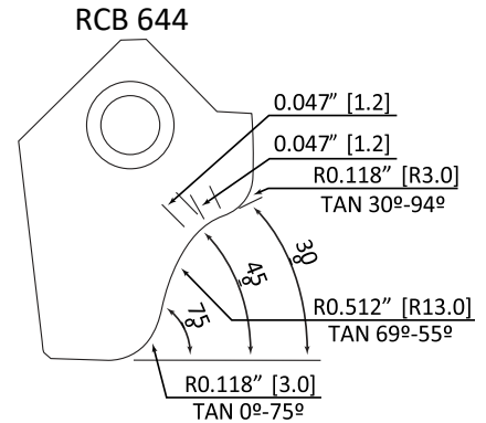
RCB644 Carbide Seat Insert R3- 30-R13-45-75-R3 / 25-12-12-30
