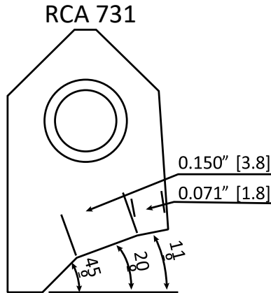
RCA731 Carbide Seat Insert 11- 20-45 / 18mm - 38mm (150")
