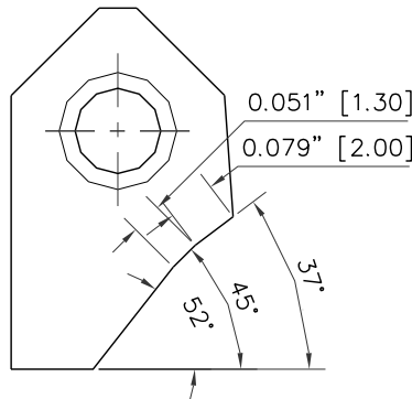
RCA005 Carbide Seat Insert 37-45-52 / 20 -13
