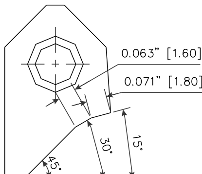
RCA307 Carbide Seat Insert 15-30-45 / 18 -16 RCA-307
