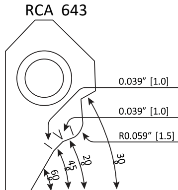
RCA643 Carbide Seat Insert 30- R15-20-45-60 / 10-10
