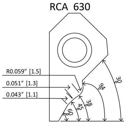
RCA630 Carbide Seat Insert 30-94-R15-38-45-60 / 13-11
