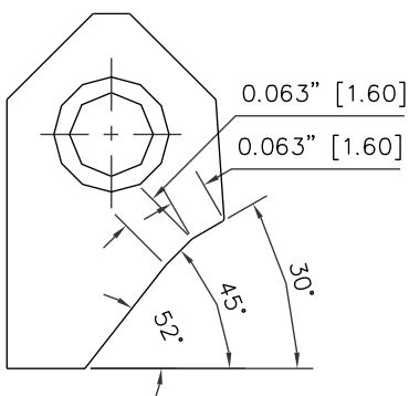
RCA016 Carbide Seat Insert 30-45-52 / 16 -16 RCA-016
