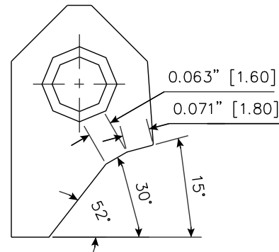
RCA308 Carbide Seat Insert 15-30-52 / 18 -16 RCA-308
