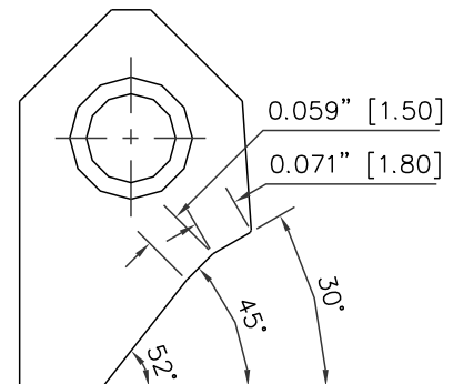
RCA009 Carbide Seat Insert 30-45-52 / 18 -15
