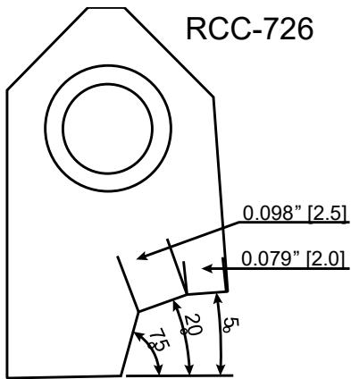
RCC726 C Blank Carbide Seat Insert 5-20-75 / 20-25
