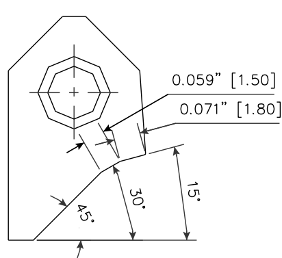
RCA304 Carbide Seat Insert 15-30-45 / 18 -15 RCA-304
