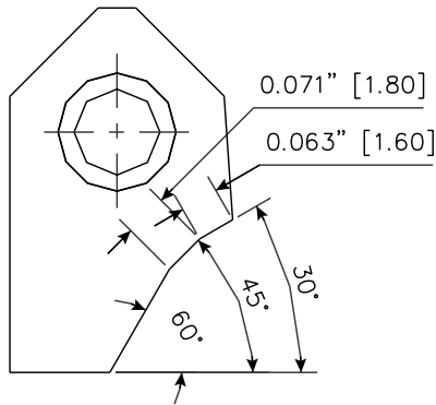
RCA049 Carbide Seat Insert 30-45-60 / 16 -18 RCA-049
