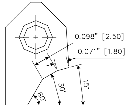
RCA328 Carbide Seat Insert 15-30-60 / 18 -25 RCA-328
