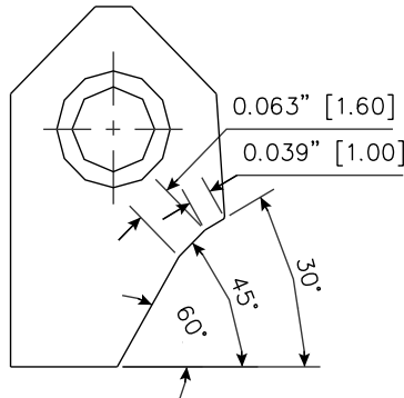
RCA047 Carbide Seat Insert 30-45-60 / 10 -16 RCA-047
