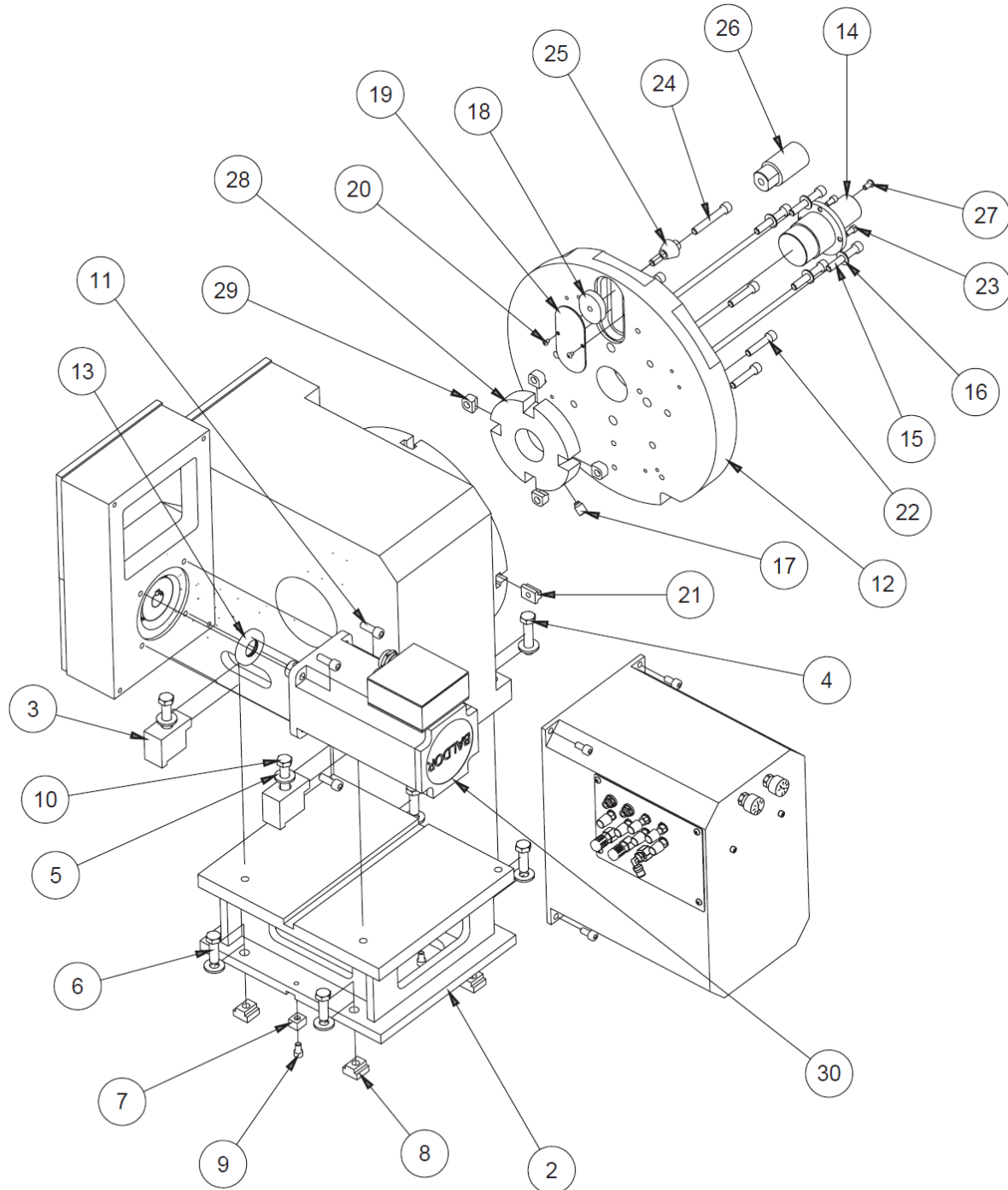
690-3-63 HEADSTOCK ASSEMBLY
